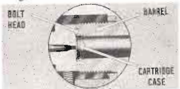
Strongest action ever developed. Cartridge case completely supported and enclosed by bolt head with no extractor cuts. And bolt head is encased in barrel. Maximum safety, accuracy.
